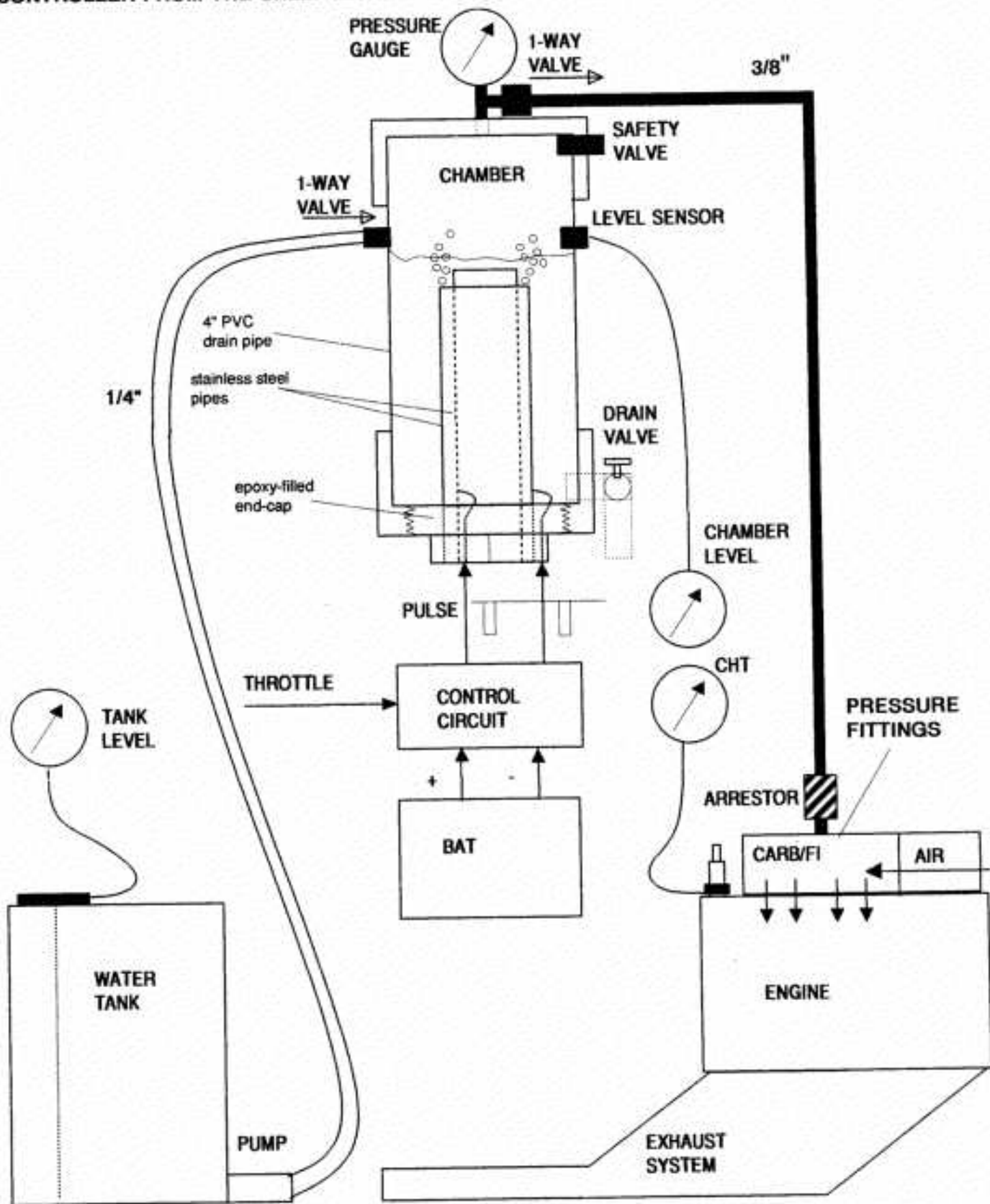
FIGURE 2 BLOC DIAGRAM
