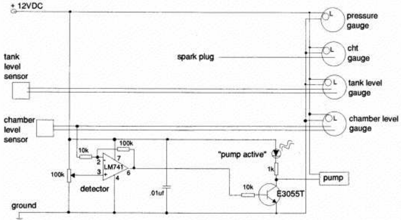
FIGURE 4 E-SCHEMATIC
